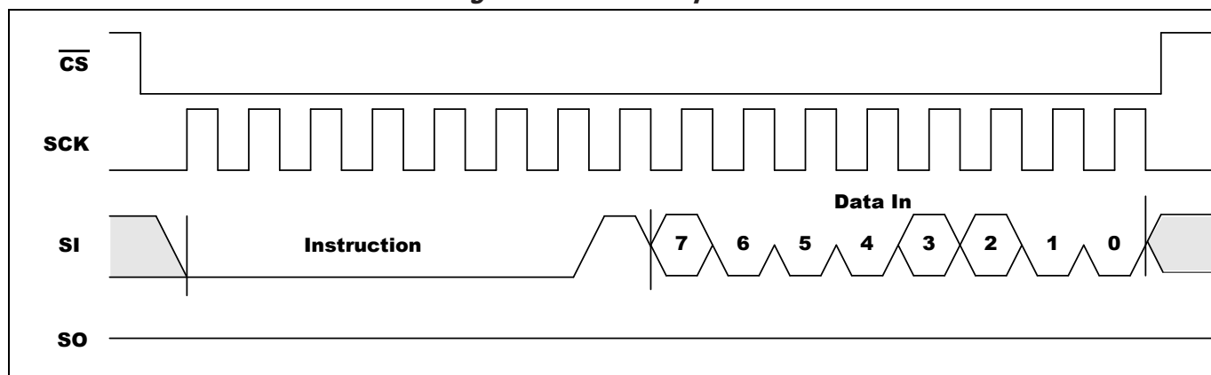
Figure 5-4. WRSR Sequence
