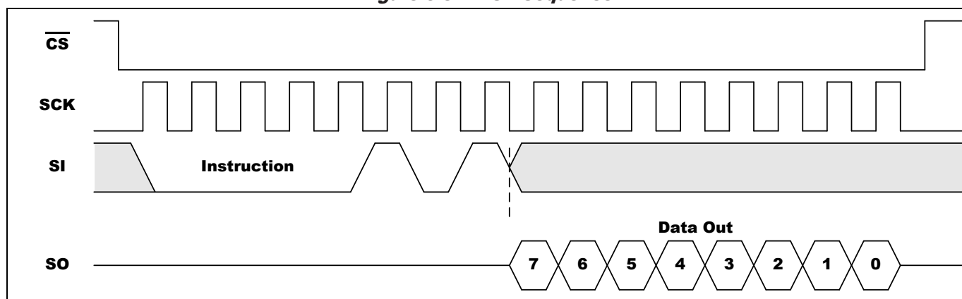
Figure 5-3. RDSR Sequence
