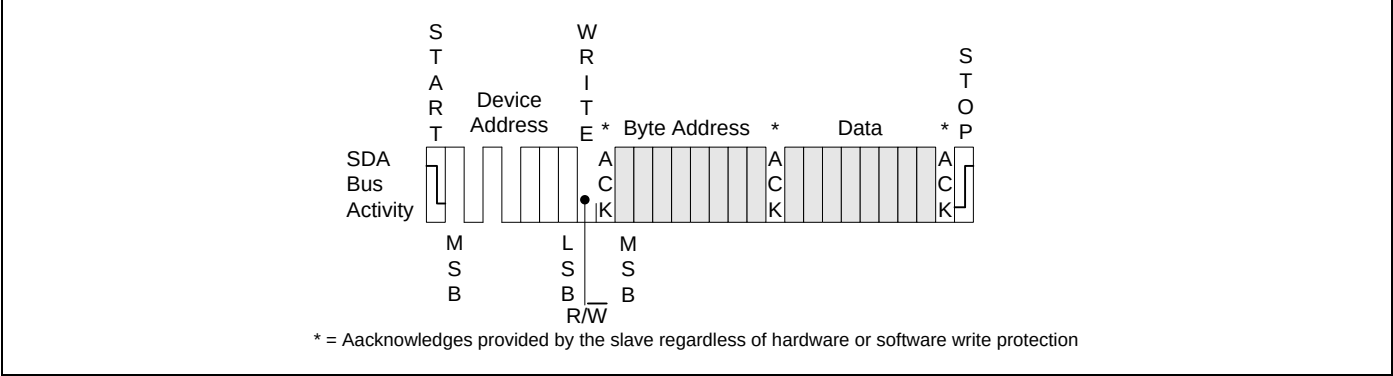
Figure 6.1 Byte Write
