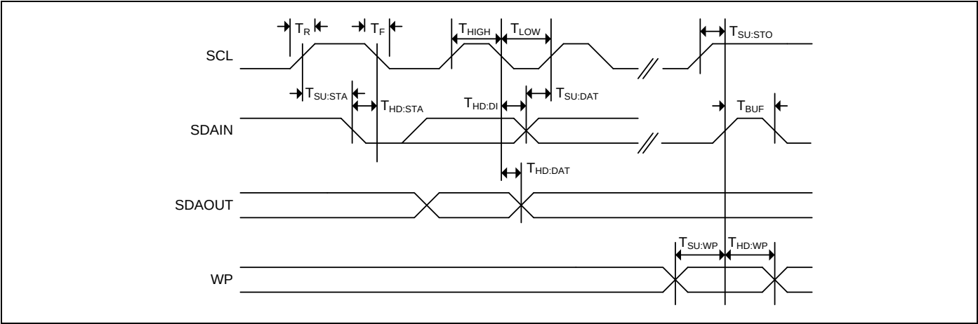
Figure 5.6. Bus Timing
