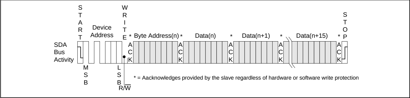
Figure 6.2 Page Write
