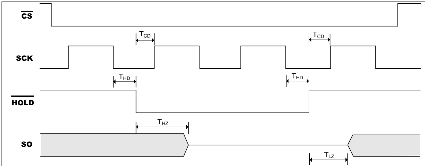
Figure 5-8. HOLD Timing
